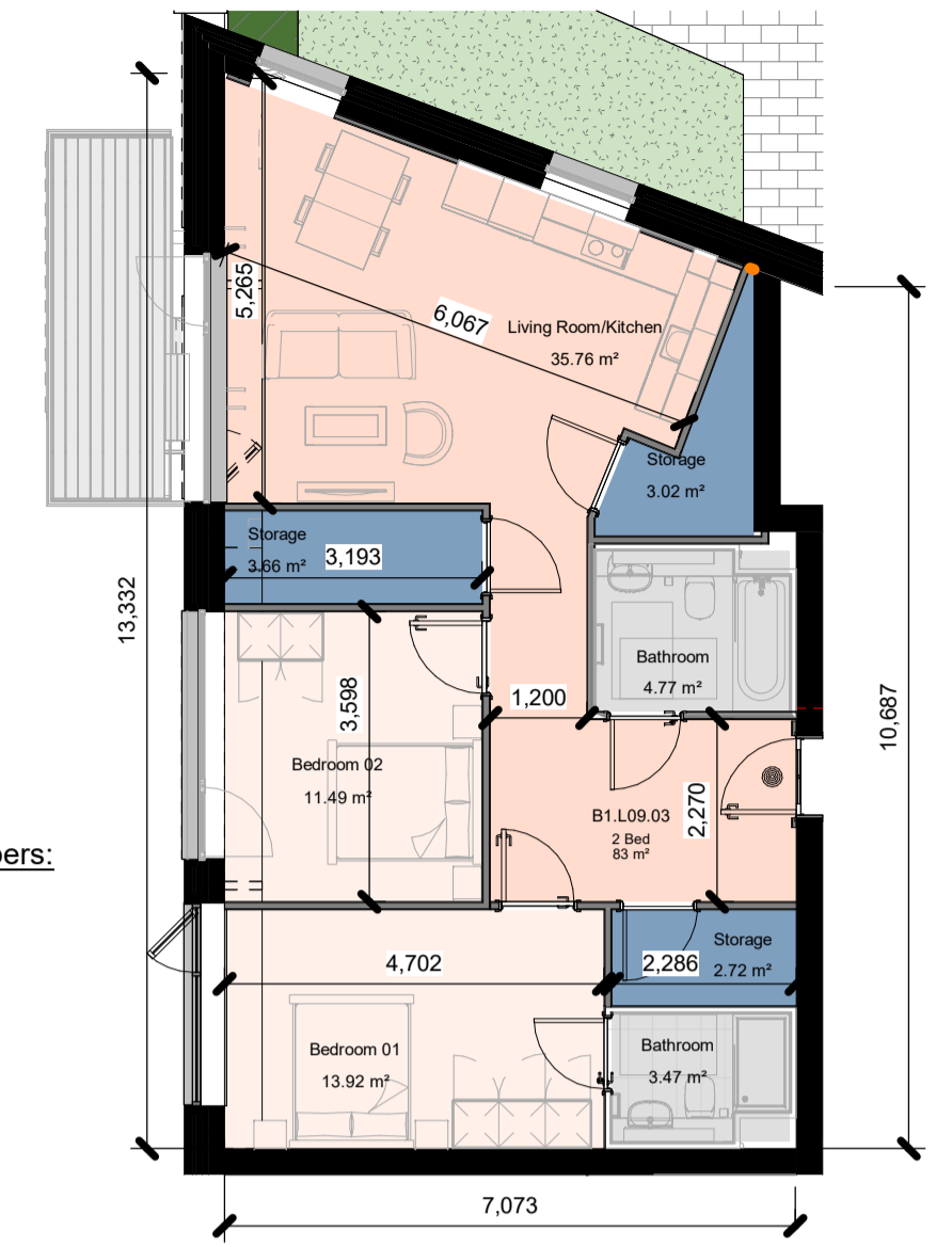
Apt Type 2 Bed (S)-9th-10th-11th Floor 1 : 100
