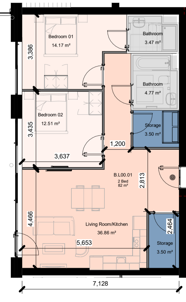
Apt Type 2 Bed (X)-Ground Floor 1 : 100
