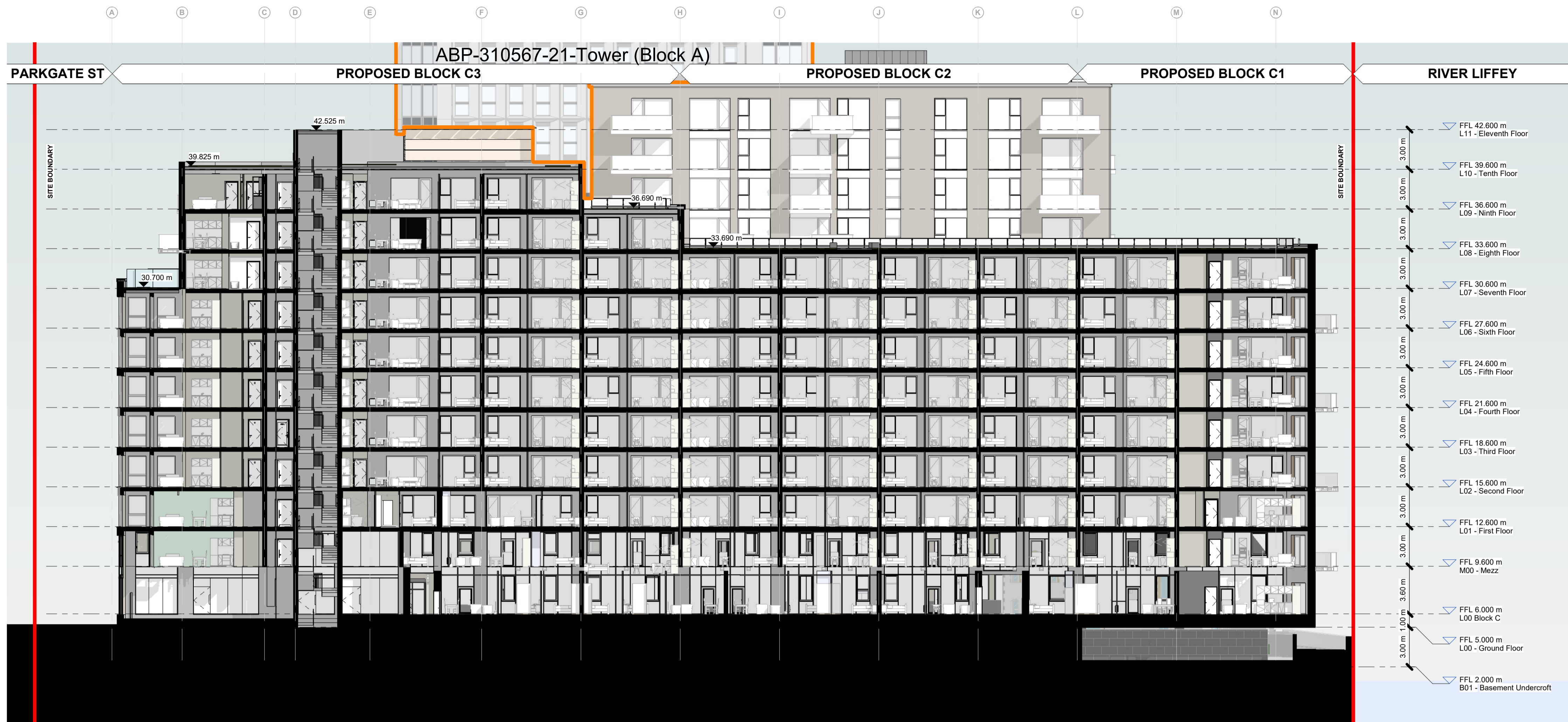
Proposed Section Block C_1-1 1 : 200
