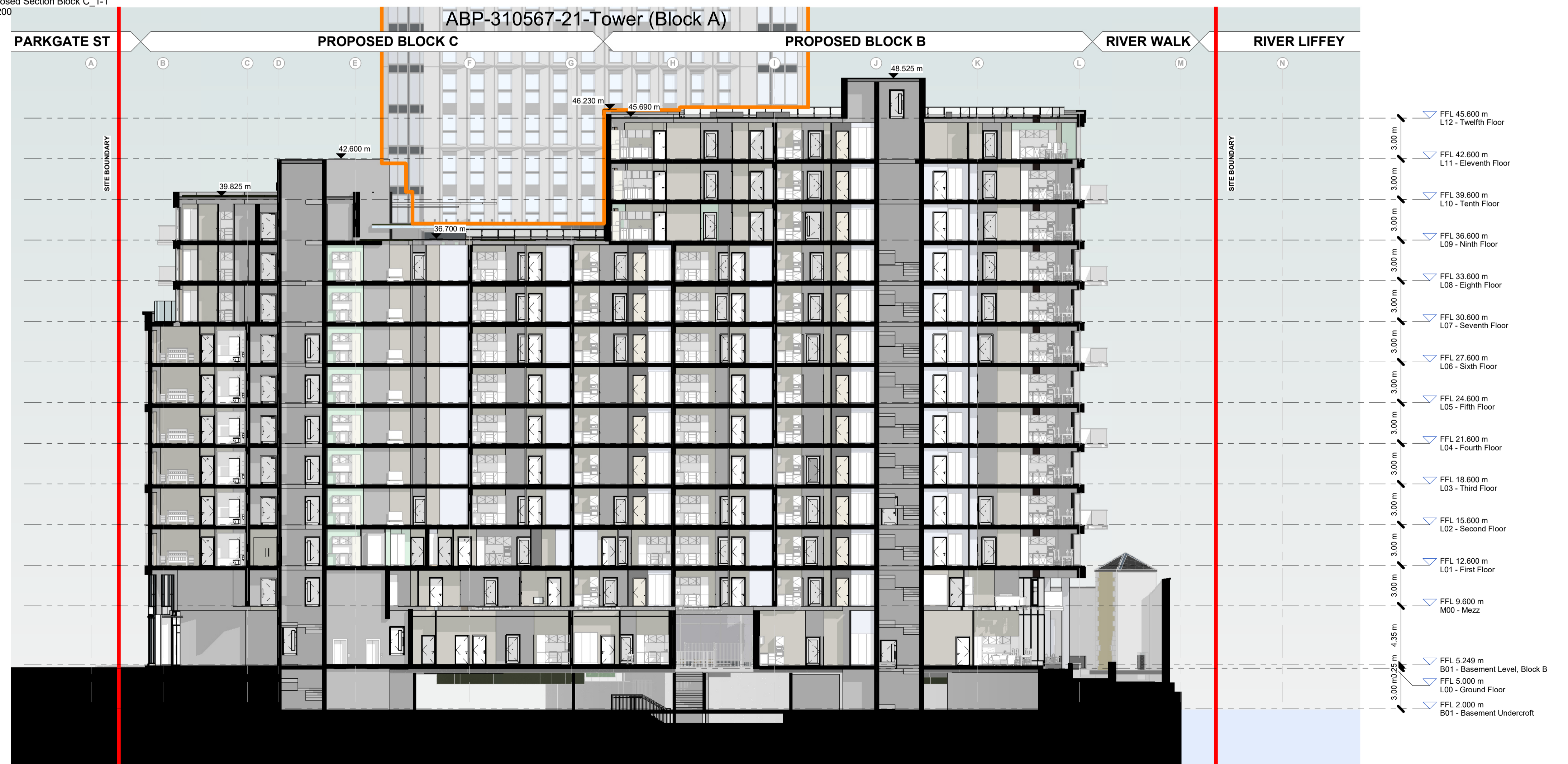
Proposed Section Block B_2-2 1 : 200
