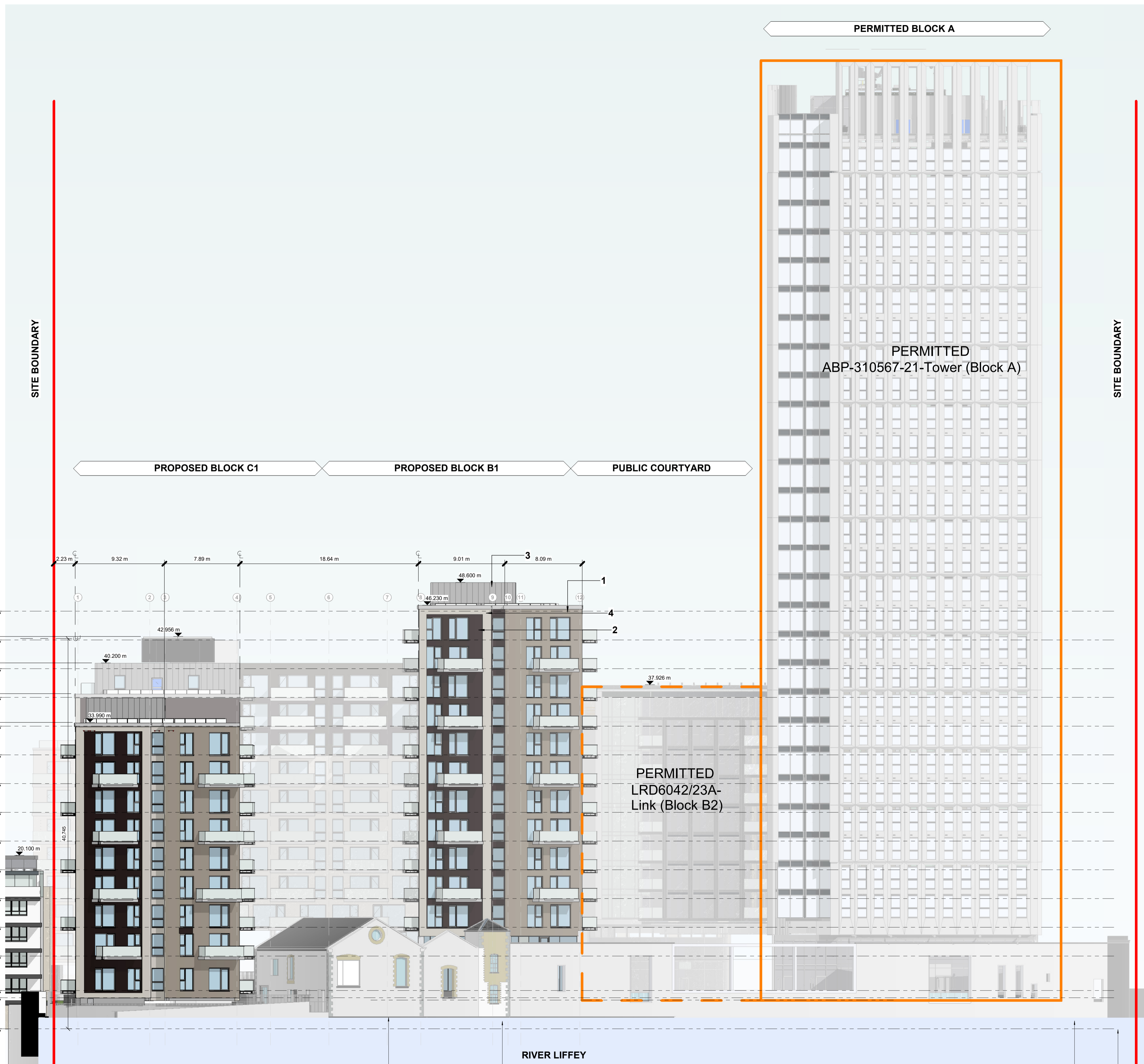
Proposed South Elevation 1 : 200
