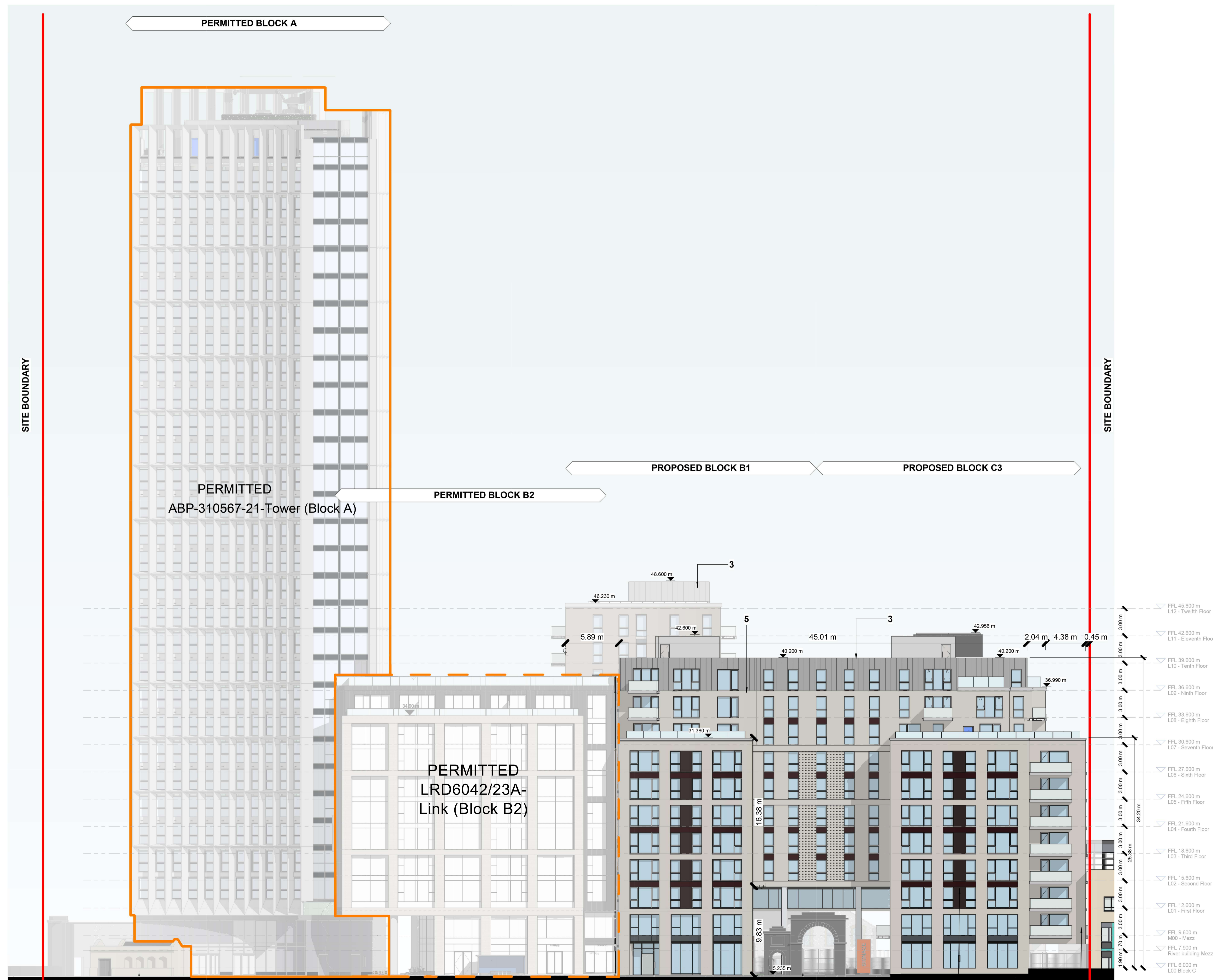
Proposed North Elevation 1 : 200
